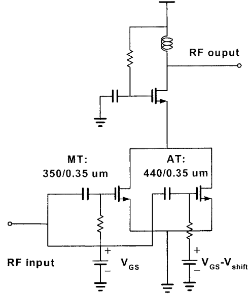
Fig. 1. MGTR with cascode configuration.
