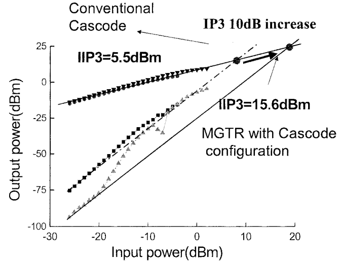
Fig. 5. IP3 comparison.
